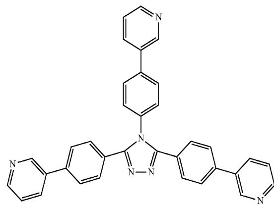
formula i
