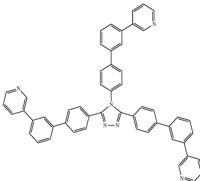
TPyBnTAZp
