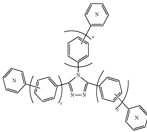
formula I
