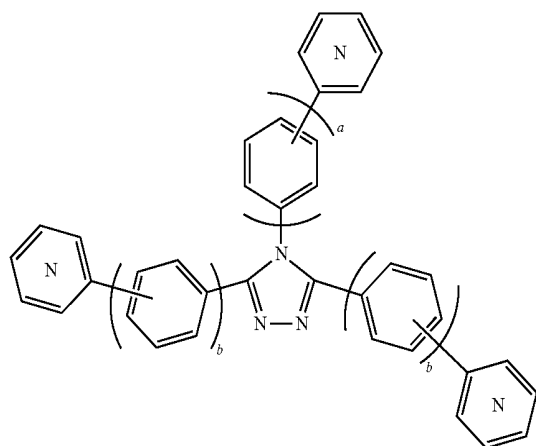
formula I
