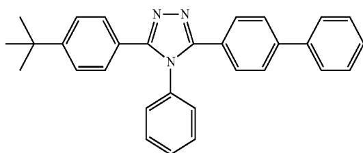
formula II
