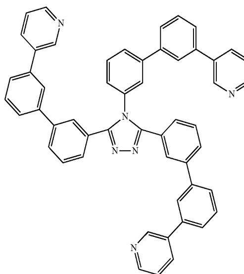
formula iv
