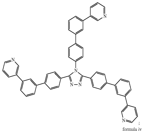
formula iv
