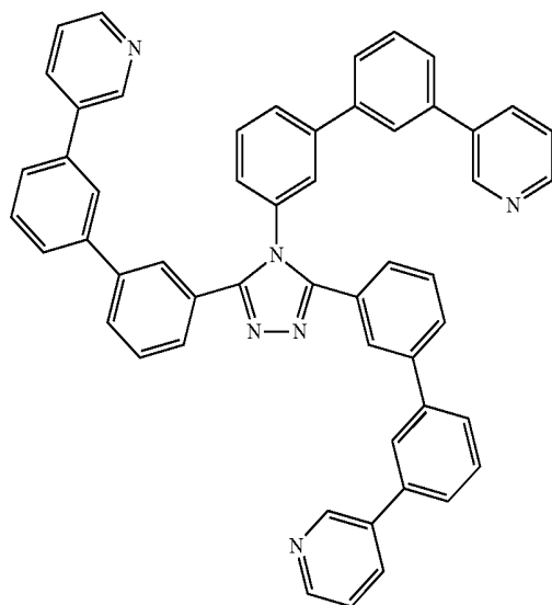
formula iv
